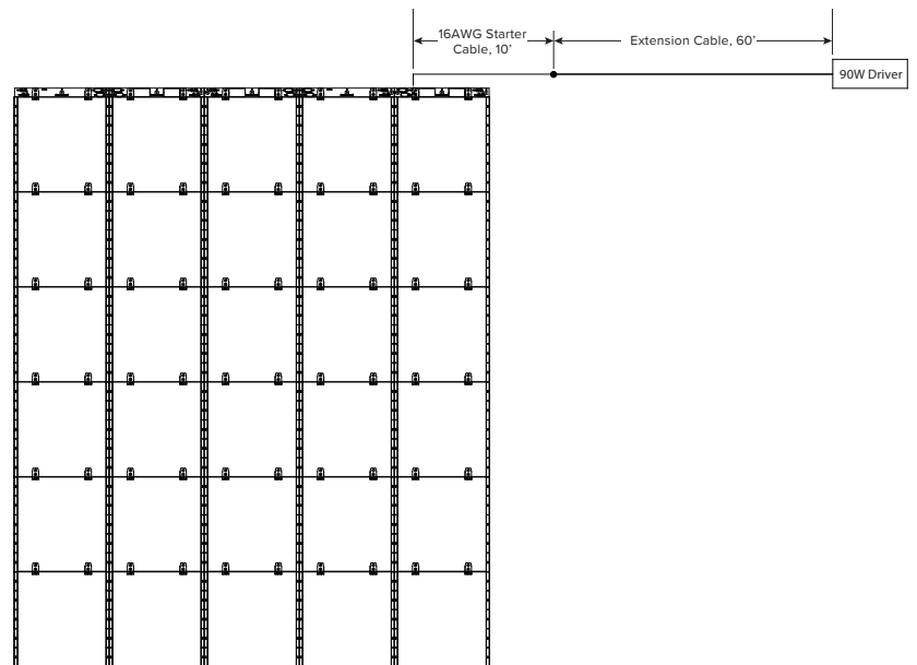
5 runs x 6 TILE-TUN-300
